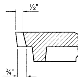
PICKSLOT DETAIL
