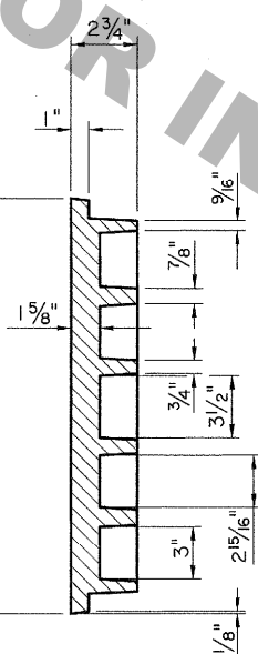
PICKSLOT DETAIL
