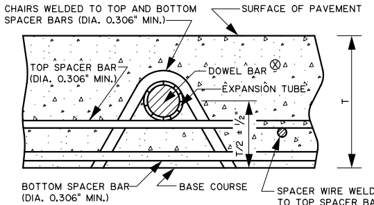
SECTION E-E SEE TABLE I (SHEET 1 OF 3)
