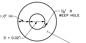
GROUT RETENTION DISK D = DOWEL DIAMETER (INCLUDING PROTECTIVE COATING)
