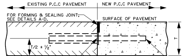
SECTION J-J TYPE BJ (TRANSVERSE BUTT JOINT)
