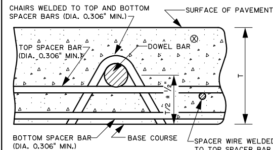
SECTION F-F SEE TABLE I (SHEET 1 OF 3)
