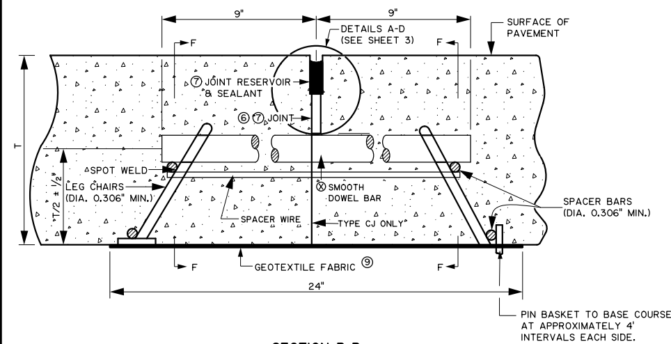
SECTION B-B TYPE TCJ OR CJ (TRANSVERSE CONTRACTION JOINT OR CONSTRUCTION JOINT) SEE TABLE I (SHEET 1 OF 3)
