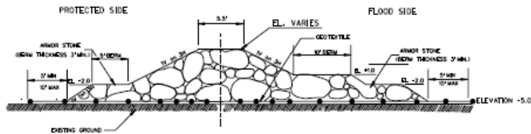
TYPICAL DISPOSAL RETENTION AND EROSION CONTROL DIKE IMAGE 3
