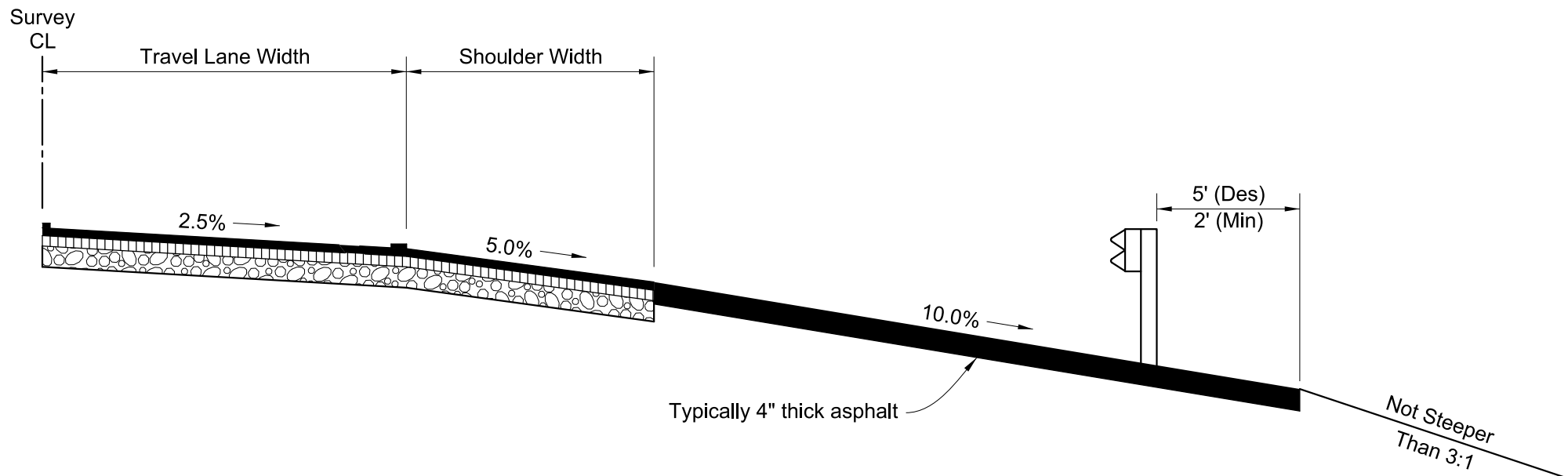
Figure 5-13: Typical Embankment Widening
