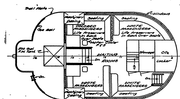
UPPER DECK
