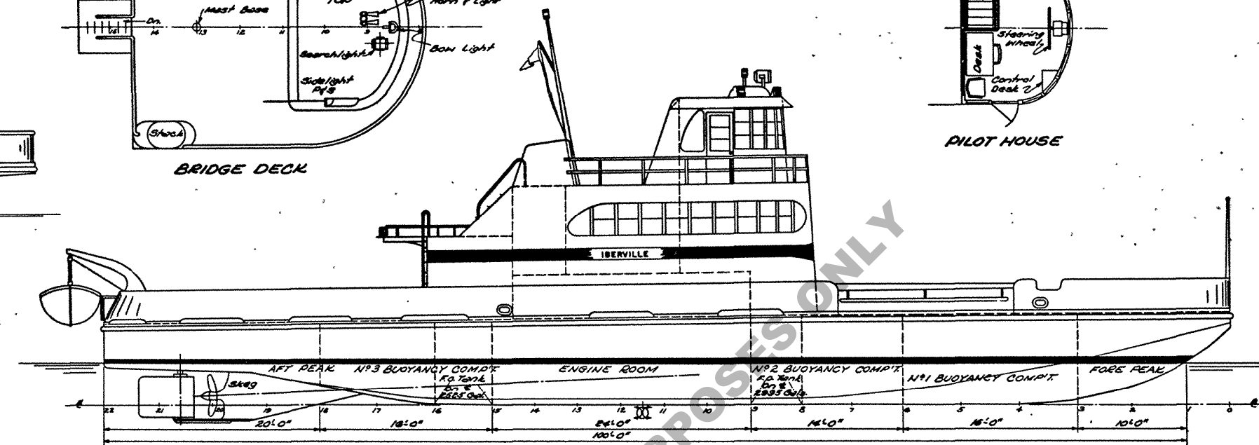
OUTBOARD PROFILE
