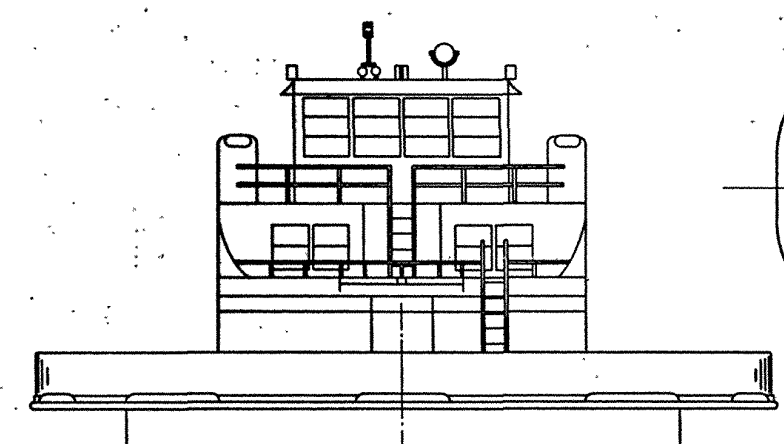
STERN VIEW
