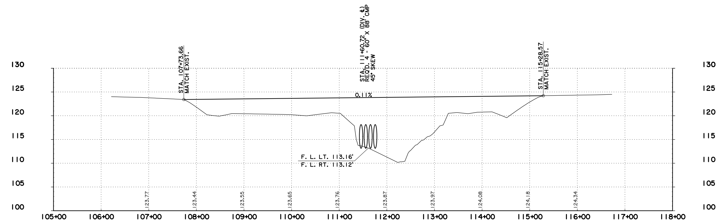
Figure 8-35: Geometric Details Diversion
