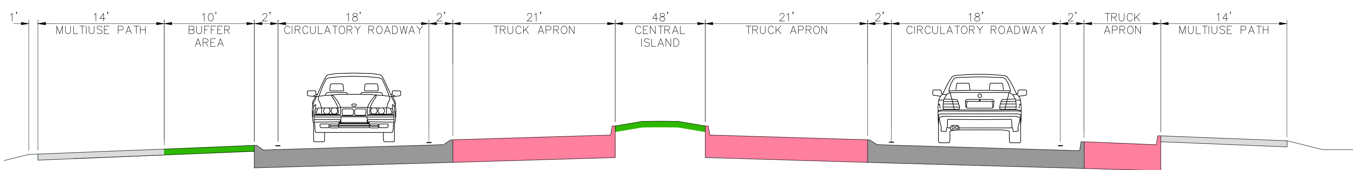
LA 1088 TYPICAL FINISHED SECTION B-B (NOT TO SCALE)
