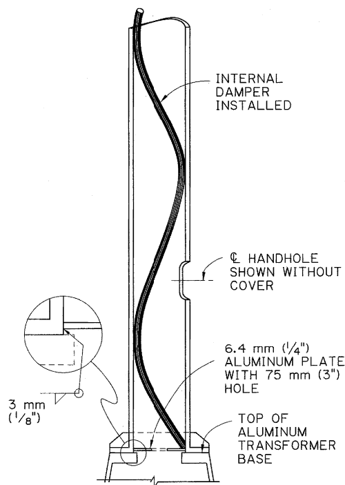
POLE SECTION
