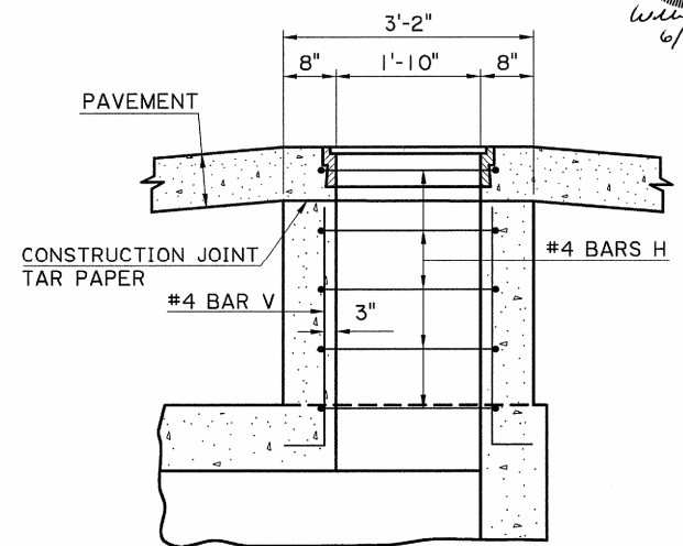
DETAIL A (MANHOLE IN PAVEMENT AREA)
