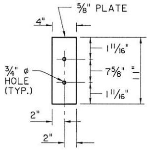
STEEL BEARING PLATE
