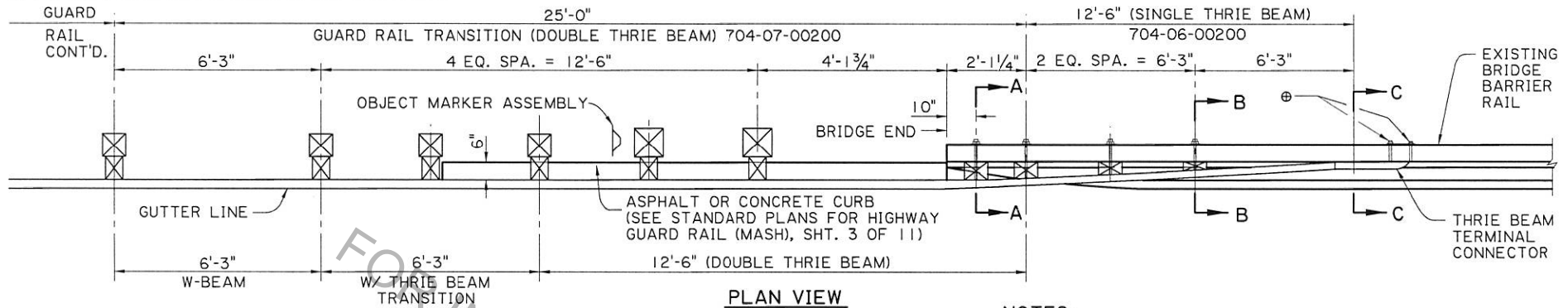
PLAN VIEW
