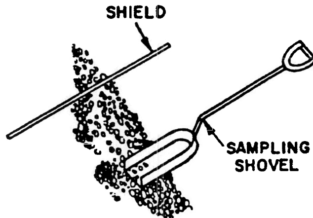
Figure 1 - Sampling Shovel
