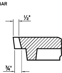
PICKSLOT DETAIL
