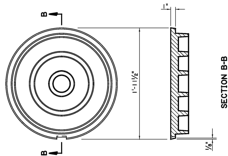
BOTTOM OF CAST IRON COVER
