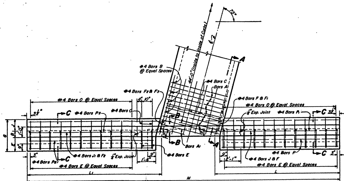
PART PLAN
