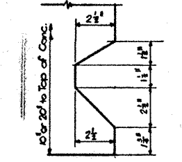
DETAIL OF SHEAR KEY FOR END FLARE
