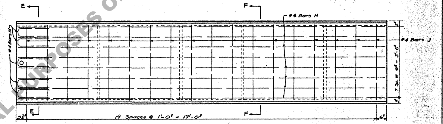
PLAN OF APPROACH SLAB UNIT SHOWING BOTTOM REINFORCING BARS
