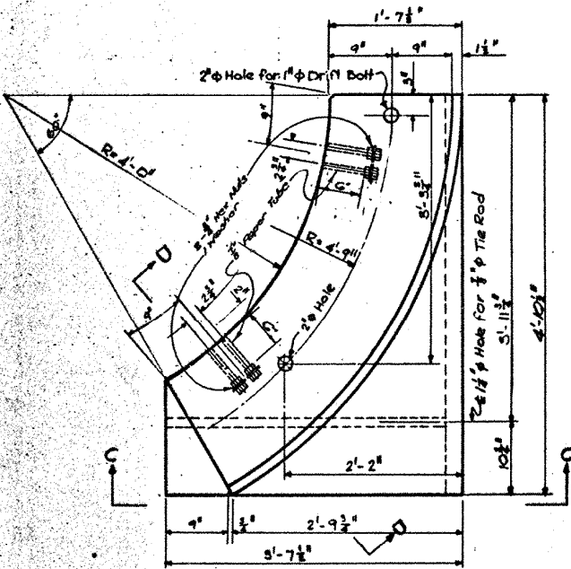
PLAN OF LEFT END FLARE Right End Flare Similar But Opposite Hand
