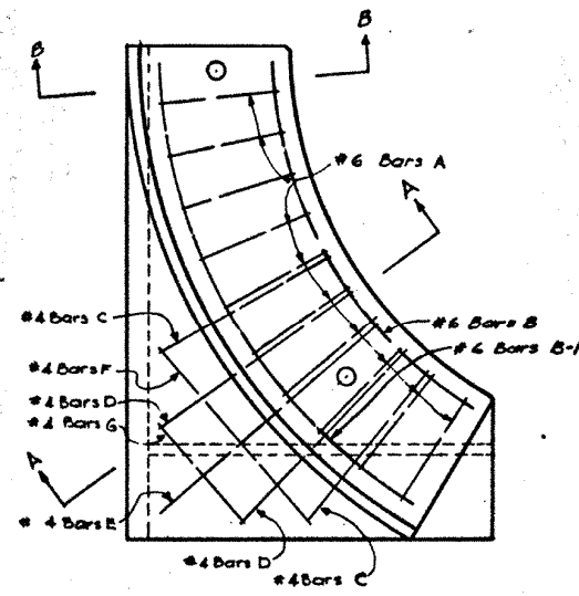
REINFORCING PLAN OF RIGHT END FLARE Reinforcing for Left End Flare Similar but Opposite Hand
