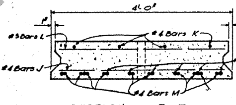
SECTION E-E
