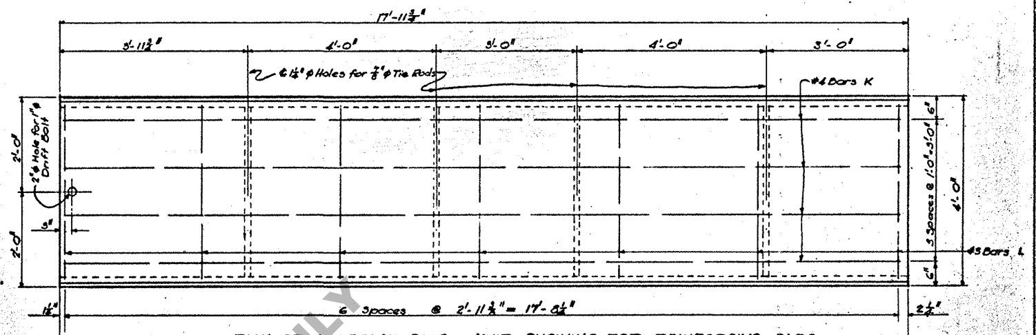
PLAN OF APPROACH SLAB UNIT SHOWING TOP REINFORCING BARS
