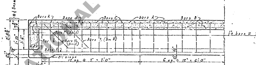
SECTION C-C Showing Reinforcement in Beams B and C
