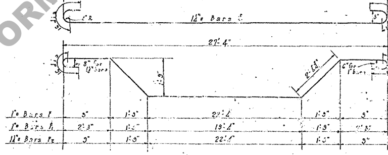
SECTION C-C Showing Reinforcement in Beams B and C
