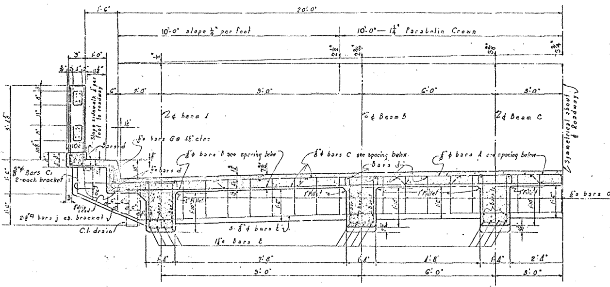
SECTION A-A Showing Reinforcement
