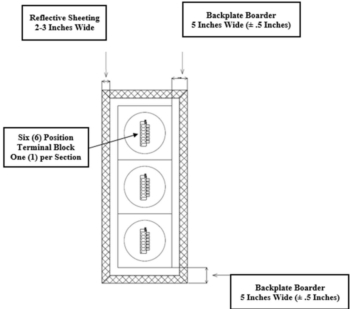
Figure 3 – Backplate and Terminal Block Details
