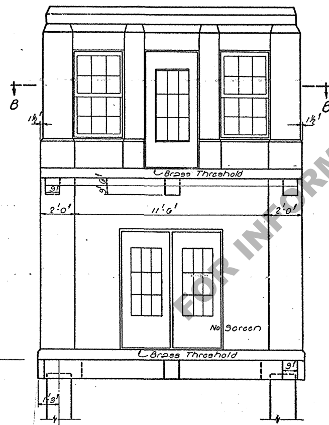
FRONT ELEVATION
