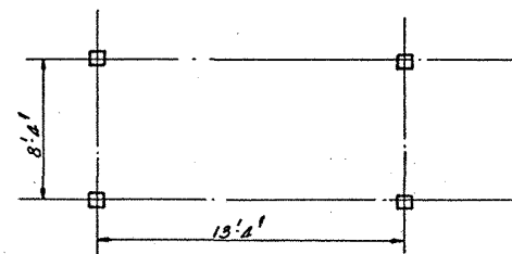
PILE SPACING PLAN
