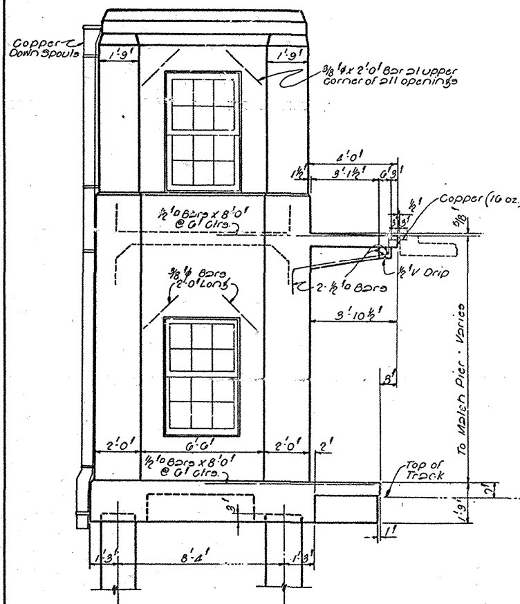
SIDE ELEVATION
