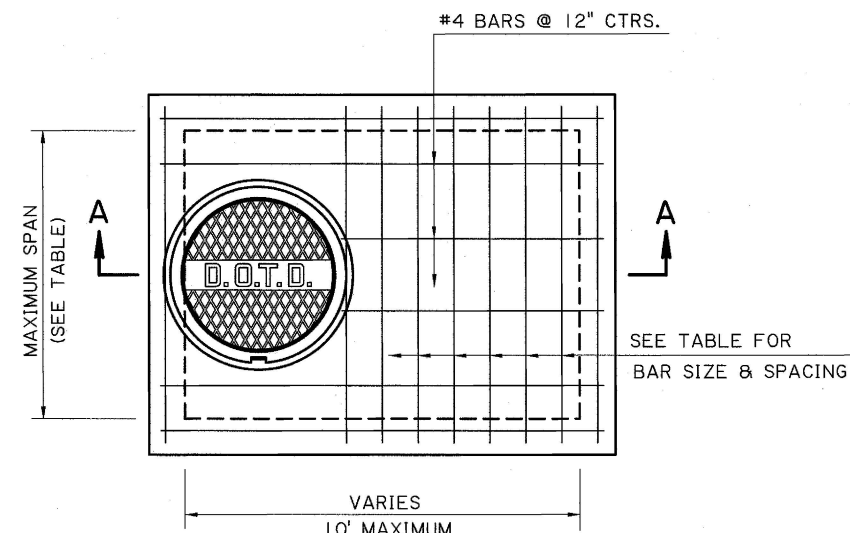
MANHOLE PLAN
