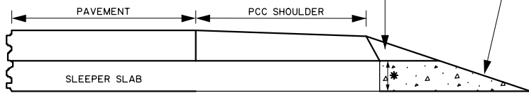
SECTION L-L (WITH CONCRETE SHOULDER)
