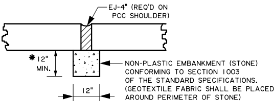
SECTION M-M (SLEEPER SLAB NOT SHOWN)
