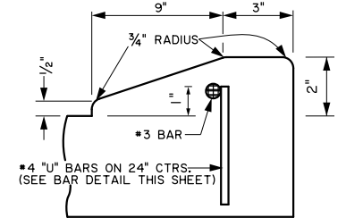
MODIFIED BARRIER OR MOUNTABLE CURB THRU DRIVEWAY
