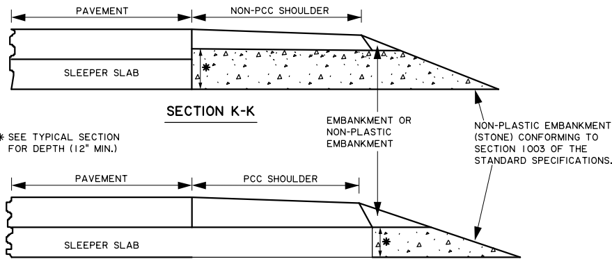
SECTION L-L (WITH CONCRETE SHOULDER)
