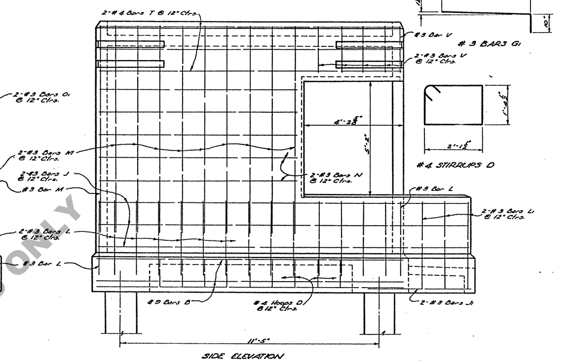
SIDE ELEVATION
