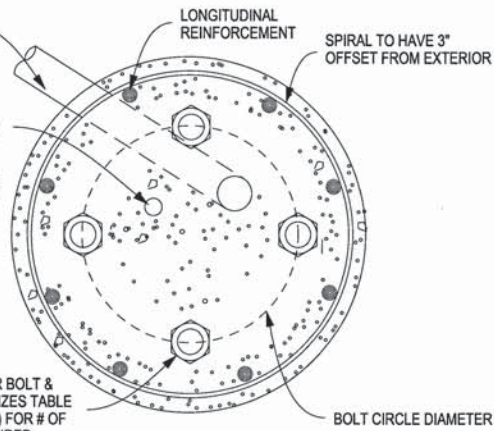
FOUNDATION PLAN NOT TO SCALE
