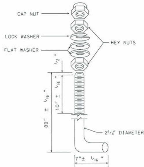
ANCHOR BOLT ASSEMBLY NOT TO SCALE
