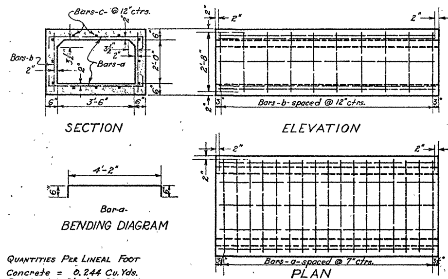
3'-6" X 2' CONCRETE BOX CULVERT
