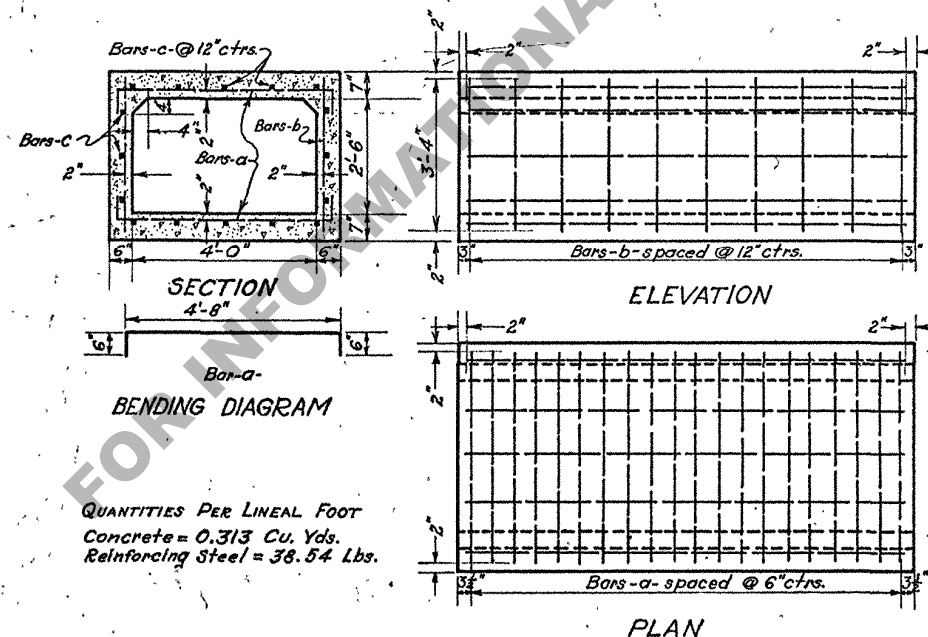
4' X 2'-6" CONCRETE BOX CULVERT
