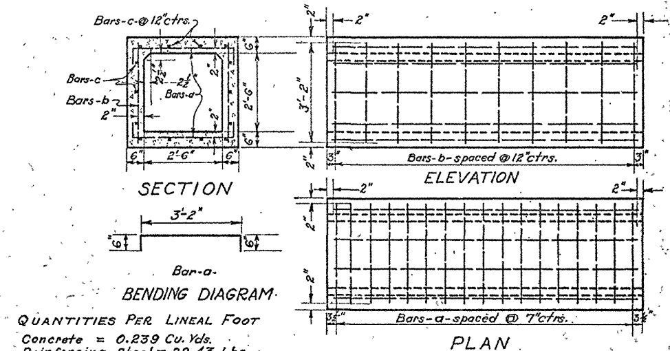
2'-6" X 2'-6" CONCRETE BOX CULVERT
