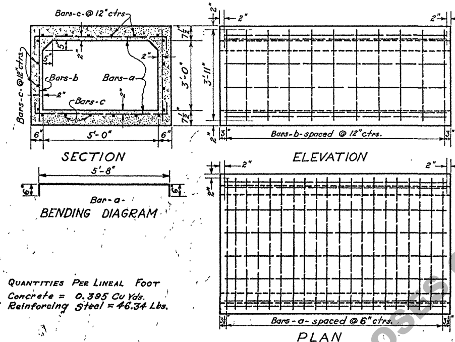
5' X 3' CONCRETE BOX CULVERT
