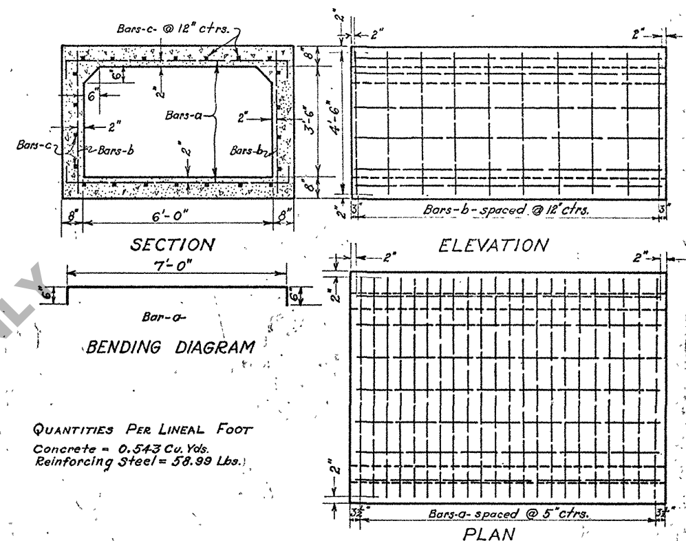
6' X 3'-6" CONCRETE BOX CULVERT
