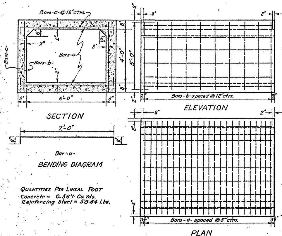
6' X 4' CONCRETE BOX CULVERT
