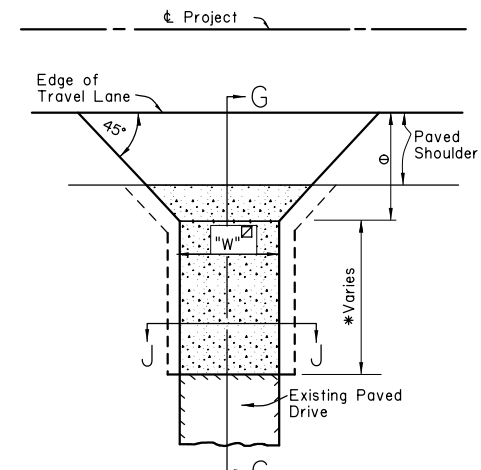
TYPE "D"
