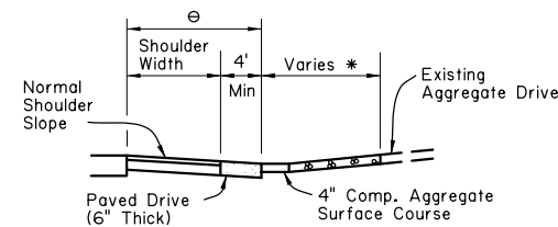
SECTION F-F
