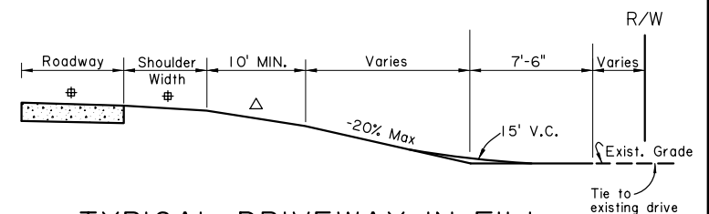
TYPICAL DRIVEWAY IN FILL
