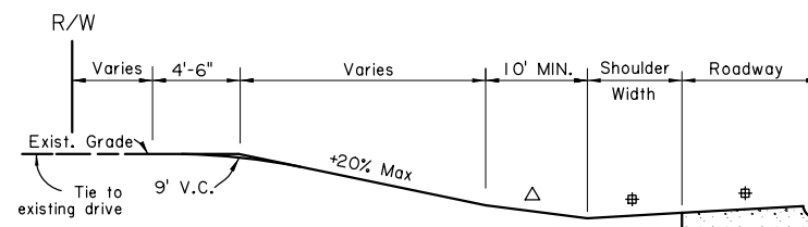
TYPICAL DRIVEWAY IN CUT
