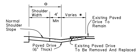
SECTION G-G
