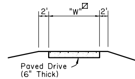
SECTION J-J
