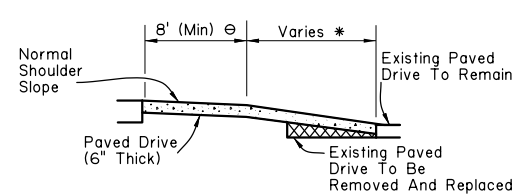
SECTION E-E
