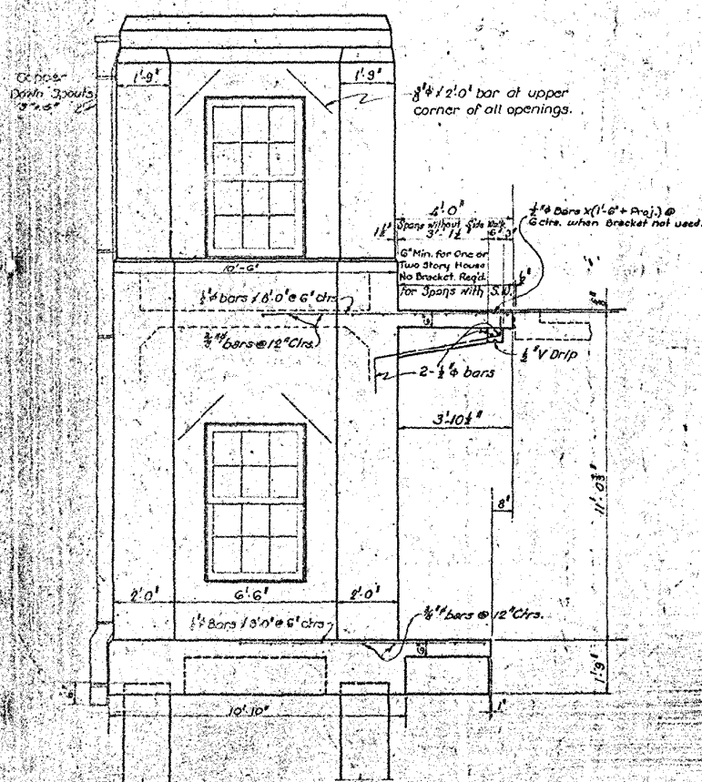
SIDE ELEVATION
