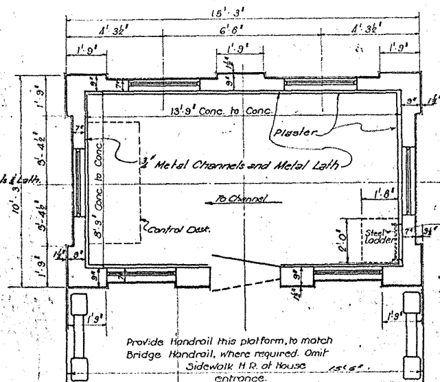
UPPER FLOOR PLAN Lower Floor Similar except for opening in floor and as shown in other views. No handrail req'd on Lower Platform. SECTION B-B
