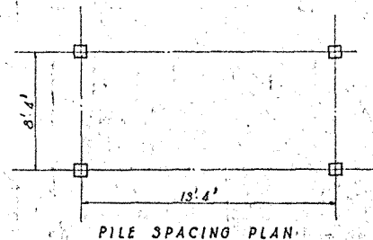
PILE SPACING PLAN
