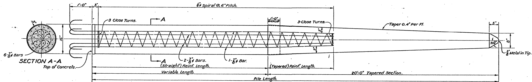
16" CAST IN PLACE METAL SHELL PILE. UNION METAL MFG. CO. FLUTED MONOTUBE PILE NO. 7 GAGE TYPE YN 16 OR EQUAL.
